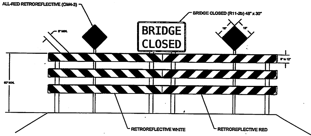
BARRICADE DETAIL
