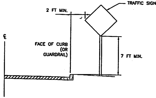
BUSINESS OR RESIDENTIAL DISTRICT (CURB & GUTTER SECTION)
